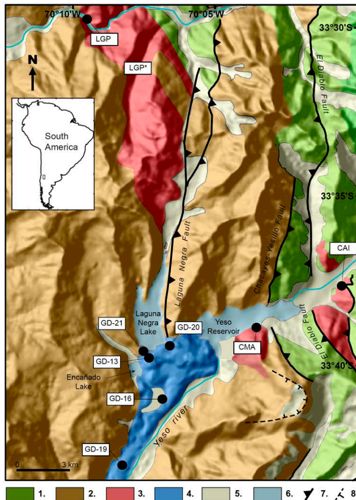
FIG. 1. Geologic map of the study area. Symboly: 1. Mesozoic rocks; 2. Oligo-Miocene rocks (Abanico and Farellones Formations); 3. plutonic rocks; 4. Mesón Alto deposit; 5. alluvial deposits; 6. water bodies; 7. faults; 8. landslide scarp; CMA=Cerro Mesón Alto Massif, LGP=La Gloria Pluton, LGP*=La Gloria Pluton (Cornejo and Mahood, 1997), CAI=Cerro Aparejo Intrusion.
