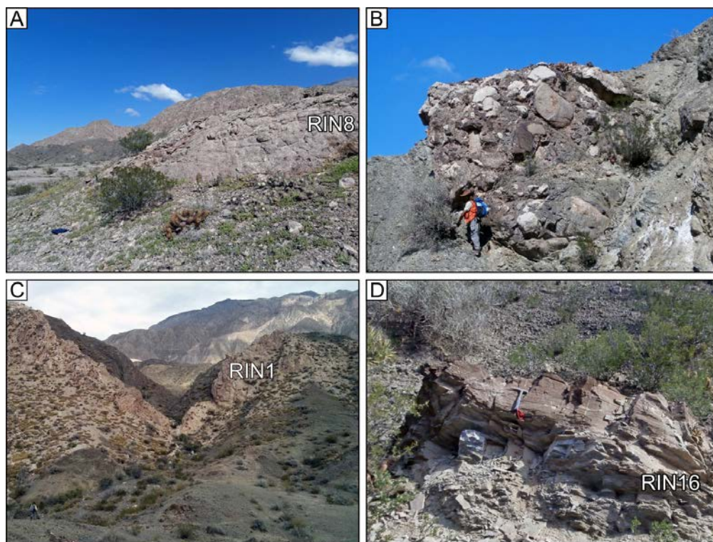
FIG. 2. Outcrops of the Rinconada mélangé in the study area, with examples of the sampled lithologies. A. Limestone block (sample RIN8); B. Conglomerate block containing rounded clasts of limestones, sandstones and of crystalline rocks; C. km-scale limestone slab of the San Juan Formation (sample RIN1) enclosed in a greenish fine-grained sandy matrix; D. dm-scale block of graptolitic quartz-arenite with calcareous cement (sample RIN16).
