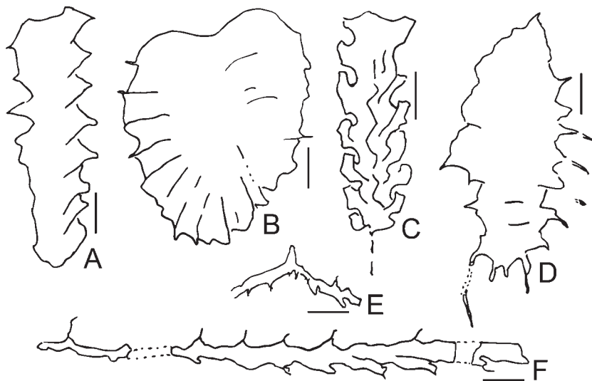
FIG. 4. Sampled graptolites from the Rinconada Formation Scale bar 0,1 mm. A. Cryptograptus schaeferi (Lapworth), CORD-MP 25805; B. Bergstroemograptus crawfordi (Harris), CORD-MP 25895A; C. Archiclimacograptus sp., CORD-MP 25895A; D. Glossograptus sp., CORD-MP 25885; E. Holmograptus spinosus (Ruedemann), CORD-MP 25827; F. Holmograptus spinosus (Ruedemann), CORD-MP 25827.
