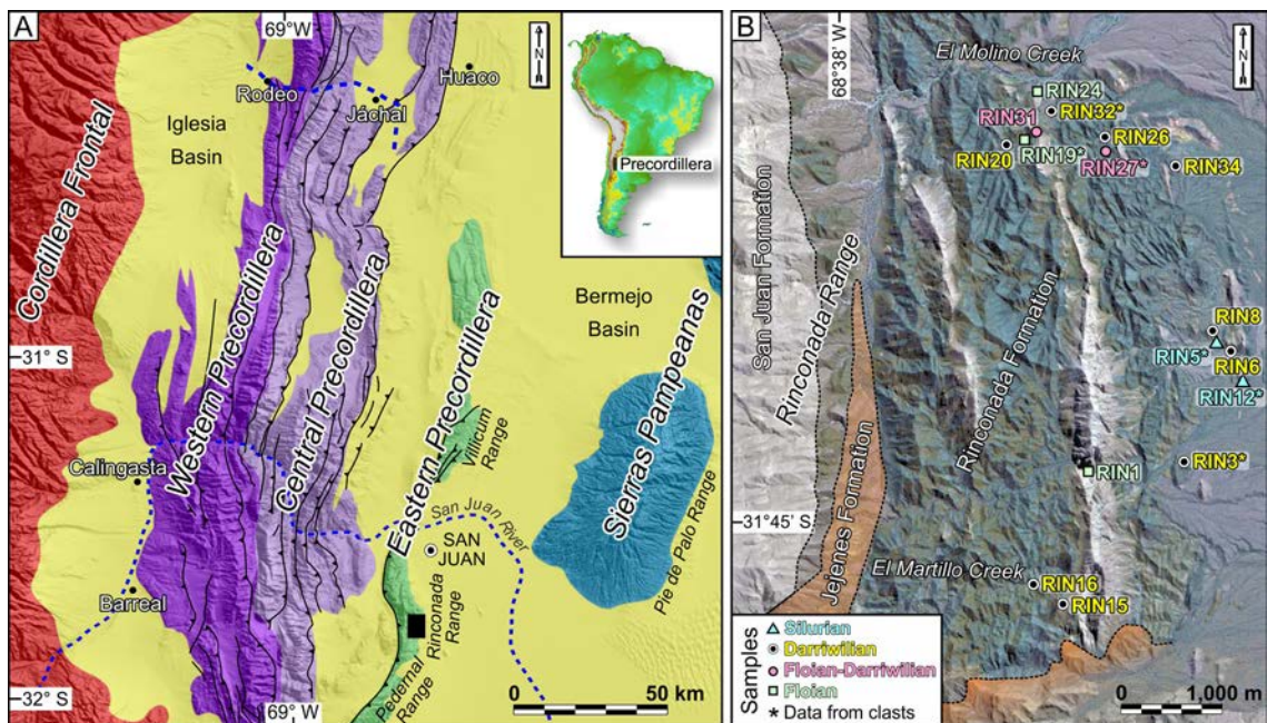
FIG. 1. A. Location map of the study area (black square), Eastern Precordillera, San Juan Province, Argentina; B. Simplified geological map of the Rinconada area showing position of the fossiliferous samples discussed in the text.
