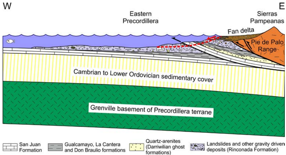
FIG. 5. Schematic cross section showing the gravity driven deposits of the Rinconada Fm being sourced by listric normal faults (red arrow) developed in the Silurian-Early Devonian eastern orogenic front (black arrows).
