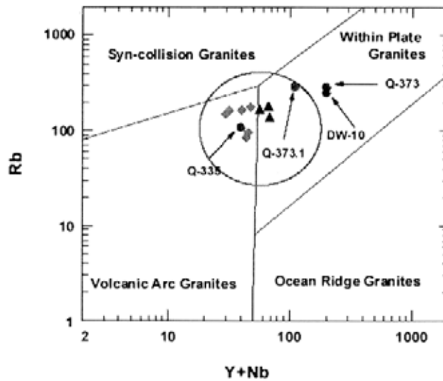
FIG. 9. Rb versus (Y+Nb) diagram (Pearce et al. , 1984) of the Tranquilo (▲), Del Salto (●) and San Lorenzo (◆) plutons. The ellipse corresponds to the Post-collision Granites field of Pearce (1996).
