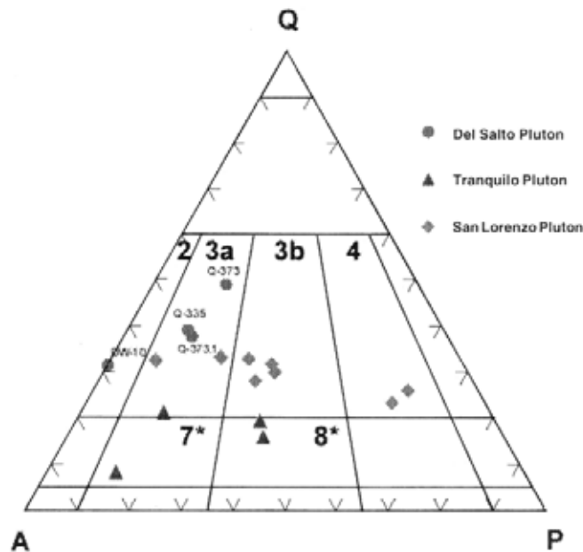
FIG. 4. QAP diagram (based on Le Maitre et al. , 1989) of the Tranquilo, Del Salto and San Lorenzo plutons. The corners of the triangle are Q =quartz; A = alkali feldspar and P =plagioclase. Field numbers are: 2 =alkali feldspar granite; 3a =syenogranite; 3b =monzogranite; 4 = granodiorite; 7* = quartz syenite and 8* = quartz monzonite.
